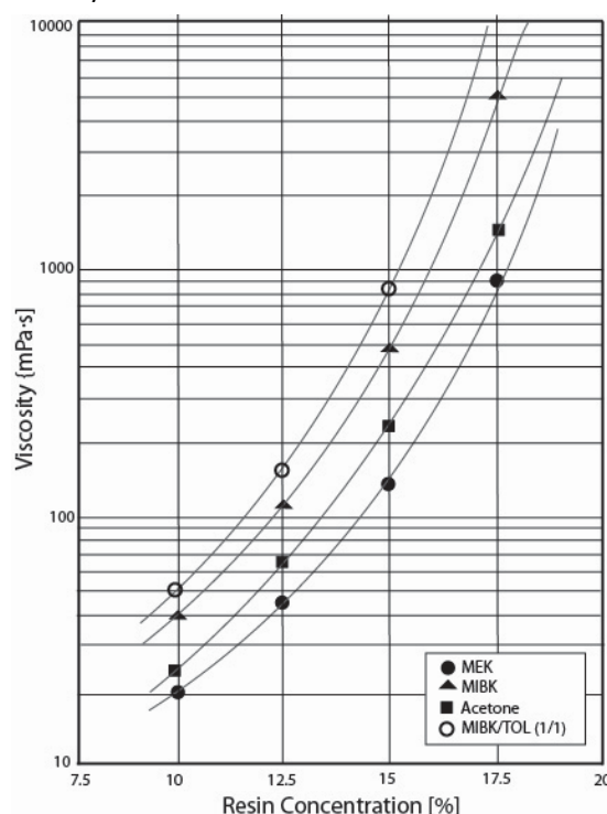
Viscosity of Solbin CN solutions with various solvents.
